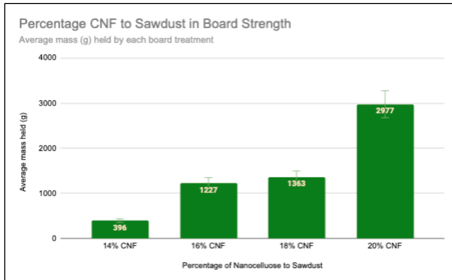
Figure 3. Representation of percentage CNF to sawdust in board strength
